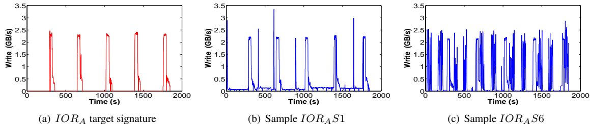
Figure 4: I/O signature of IOR_A and two samples
