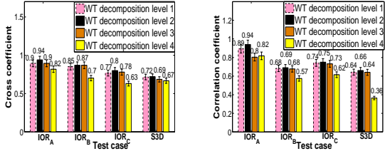
Figure 17: IOSI - WT sensitivity analysis
