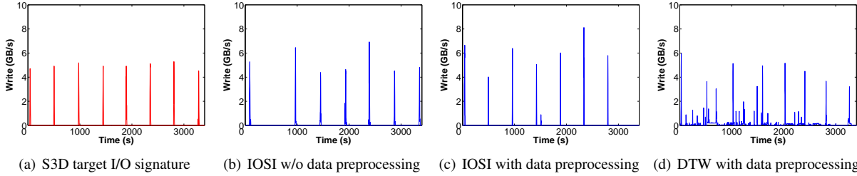
Figure 15: S3D target I/O signature and extracted I/O signature by IOSI and DTW
