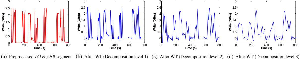
Figure 9: dmey WT results on a segment of IORAS6
