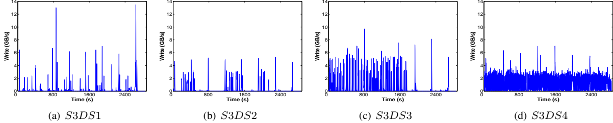
Figure 14: S3D samples
